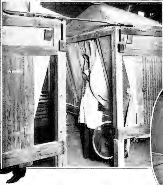
At Left, the Hopper Where the Workman Operates. A Strong Suction Saves the Sand and Draws Off the "Flour" So Dangerous to the Lungs
